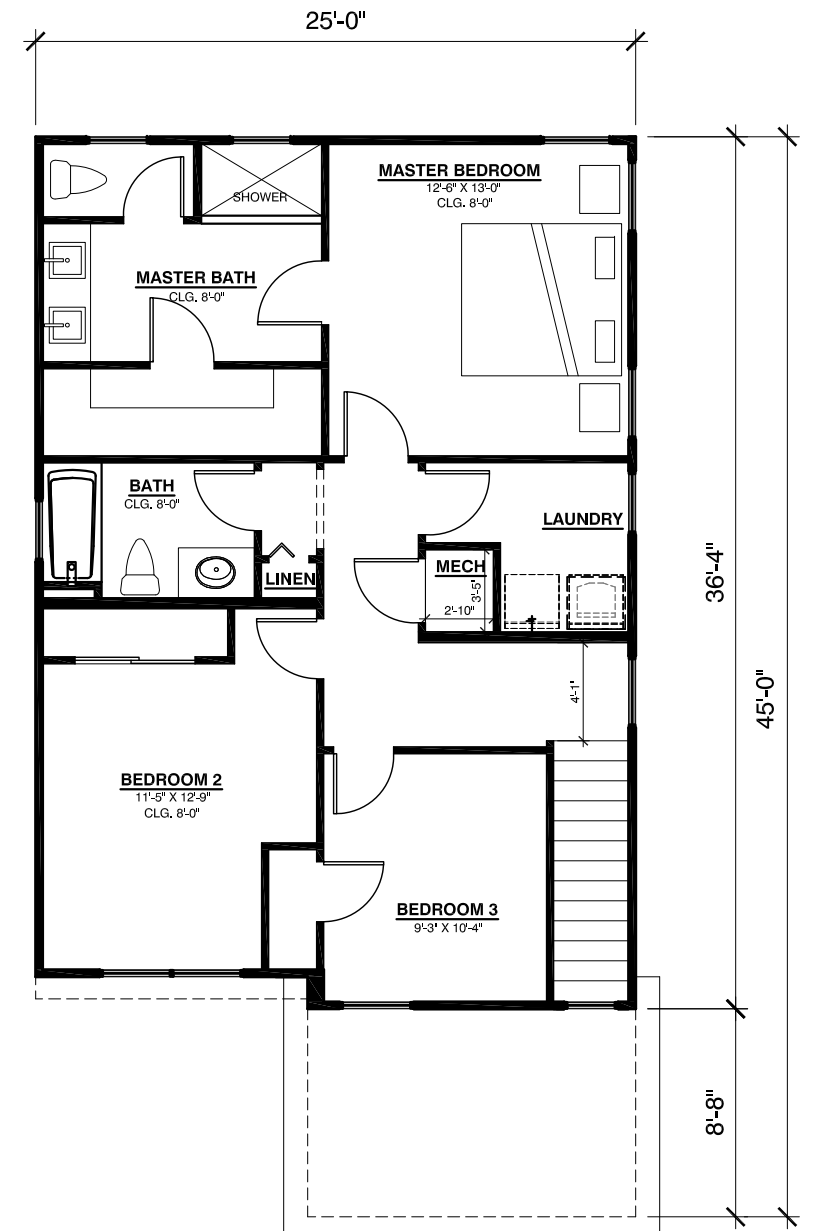
SECOND FLOOR PLAN CONDITIONED AREA 845 SF MECHANICAL ROOM 10 SF TOTAL SQ.FT. 855 SF
