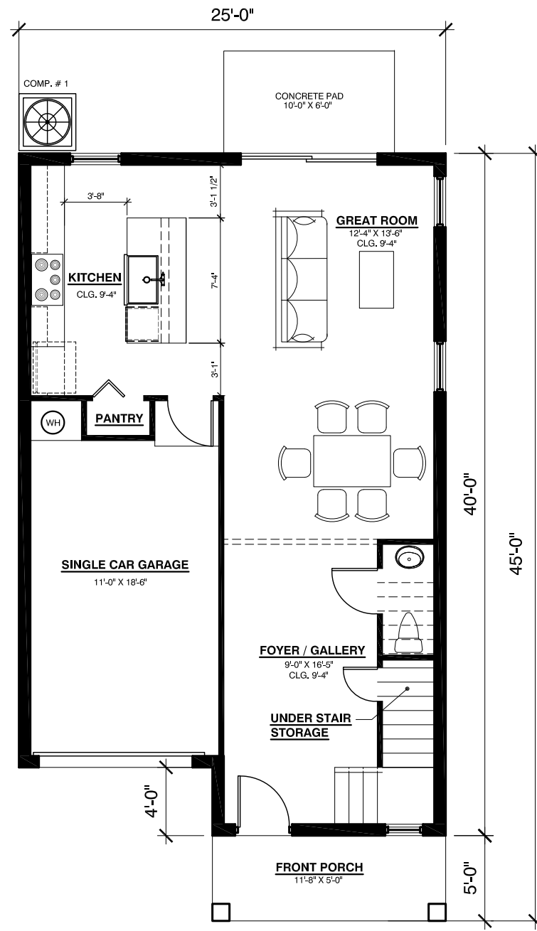
FIRST FLOOR PLAN CONDITION SPACE 713 SF GARAGE 241 SF FRONT PORCH 68 SF TOTAL 1022 SF
